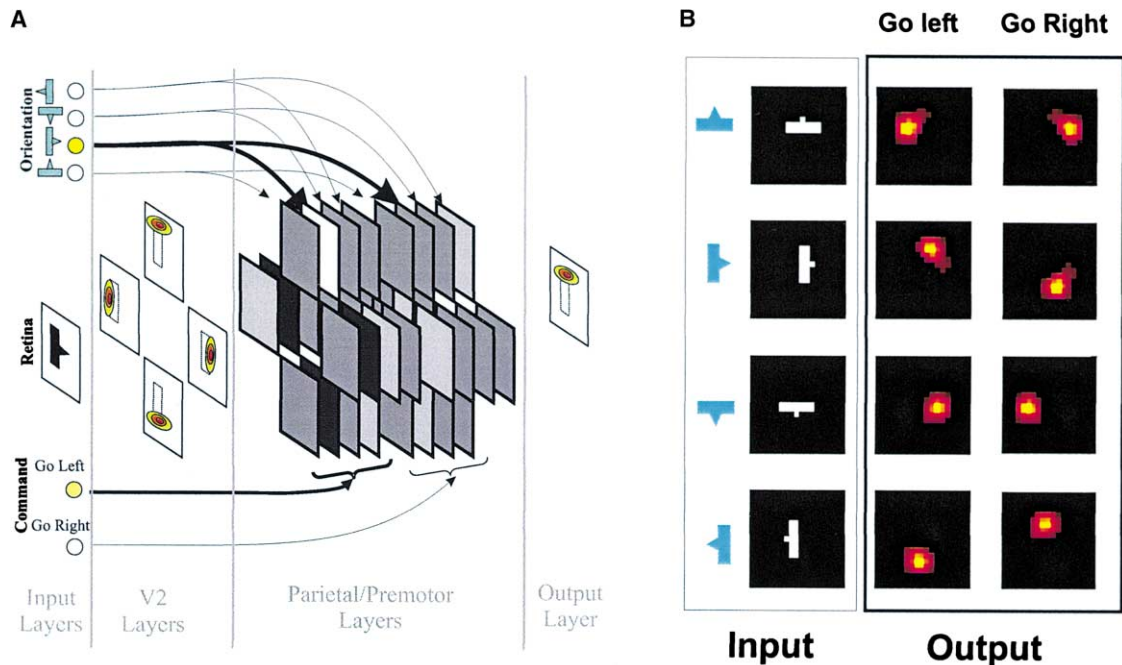
Figure 3. Network Architecture
